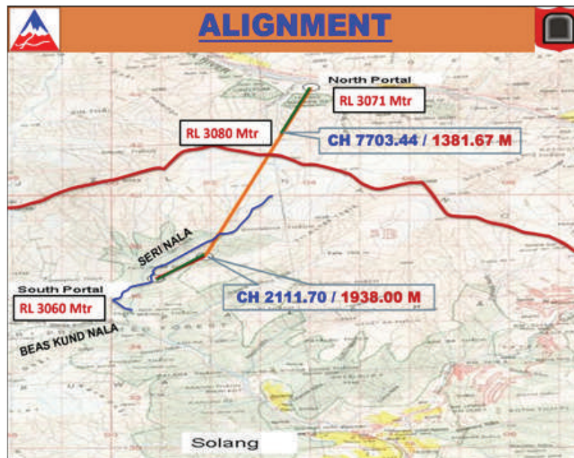
Figure: Atal Rohtang Tunnel-Location and Alignment
