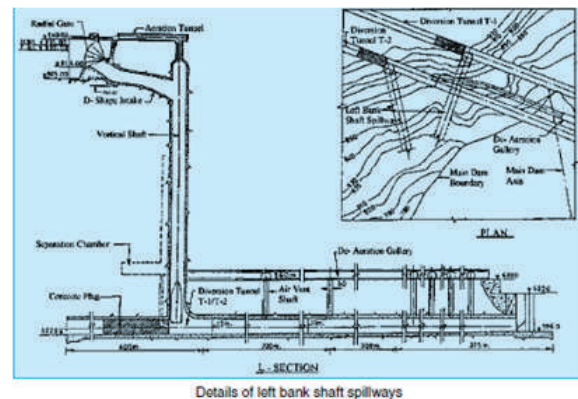
Figure: Details of left bank shaft spillways
