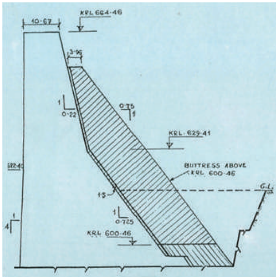
Figure: Section of Strengthened Koyna Dam after 1967 Earthquake
