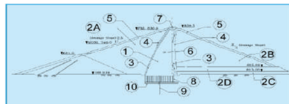
Figure: Typical Section of Tehri Dam
