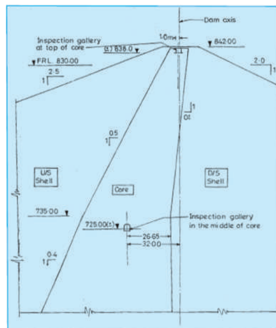
Figure: Mid-level Inspection gallery & Top Level Inspection Gallery in Dam Section
