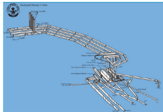
Figure: The model perspective projection of the entire power house
