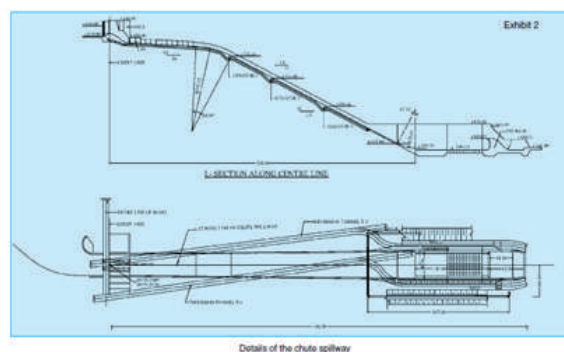
Figure: Tehri Chute Spillway – Section showing aeration arrangements and stilling basin on faulty foundation with special provisions
