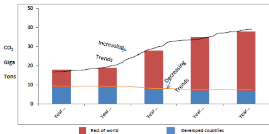
Fig. 2 (ii) : Trend of CO 2 since 1990
