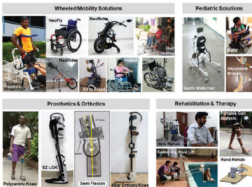
Fig. 11: Prototypes of assistive and rehabilitation devices developed at R2D2 over the past 10 years
