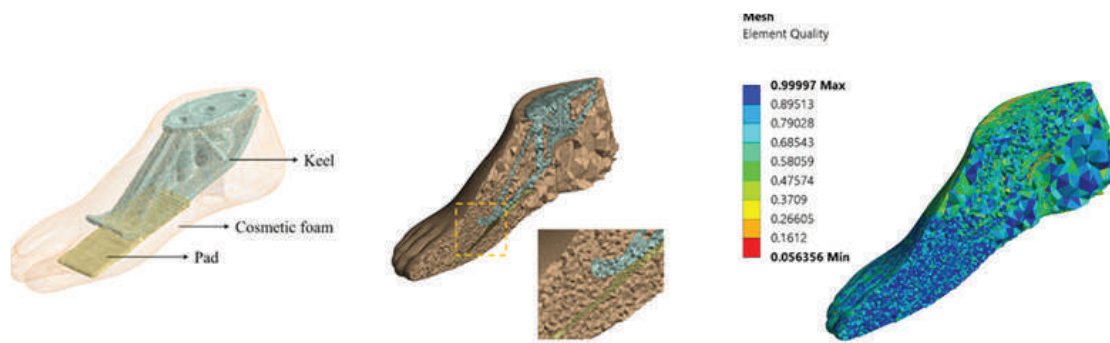
Fig. 8 : Geometry of a solid Ankle cushioned heel (SACH) foot from 3D scanning and processing and its corresponding meshed finite element model
