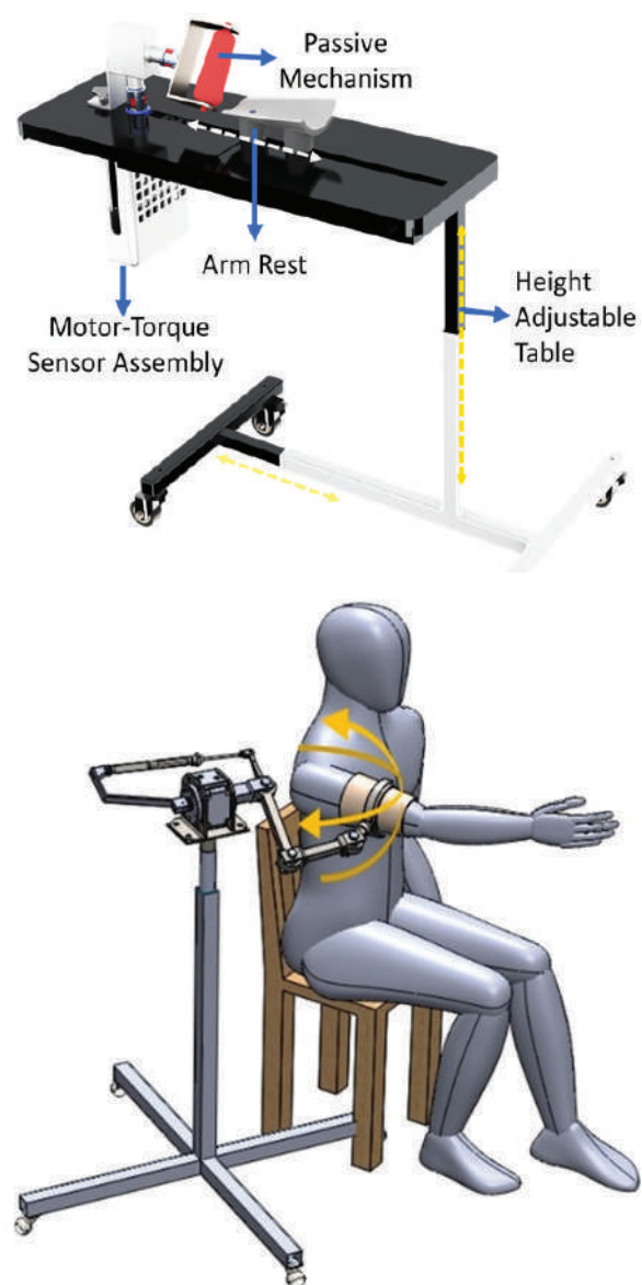
Fig. 7 : Device for (a) Hand neurorehabilitation and (b) Arm neurorehabilitation
