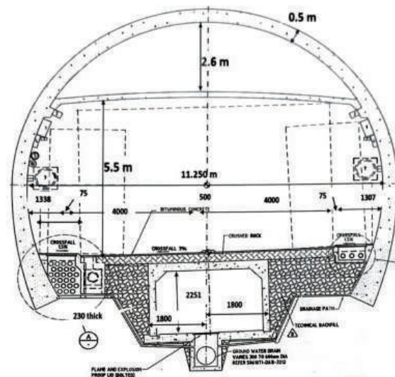
Figure: Cross section of the tunnel
