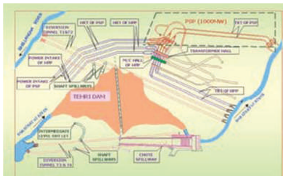
Figure: Depiction of Project layout
