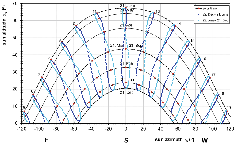
Fig. 4.30 Cylindrical type of solar-path diagram designed for Ljubljana ( L 46.1°, \lambda -14.5°) [14]. The difference between solar and civil time when ET is 0 is only 2 min because Ljubljana lies close to the standard time-zone meridian. The sun path shown for the 21st February corresponds for 21st October; the analemmas are coloured with light blue colour for the period between 22nd June and 21st December and by dark blue colour line for the period between 22nd December and 21st June (solar noon will be at ~ 11:50 civil time on 21st October and at ~ 2:15 on 21st February. Note the summer time not taken into account)
