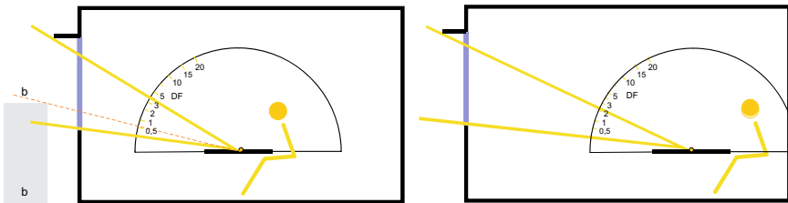
Fig. 4.56 A protractor is a simple graphical tool to determine the sky component daylight factor. The DF is determined as the difference between the DF read from tool for the angles subtending the point's view of the sky
