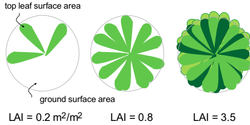
Fig. 1.61 Leaf area index LAI is the ratio of the total plant leaf top surface area to the surface area of the ground beneath the plant. Typical values are between 0 for barren ground and 8 \text{ m}^2/\text{m}^2 for thick woods. The LAI of grassy land is 1 \text{ m}^2/\text{m}^2
