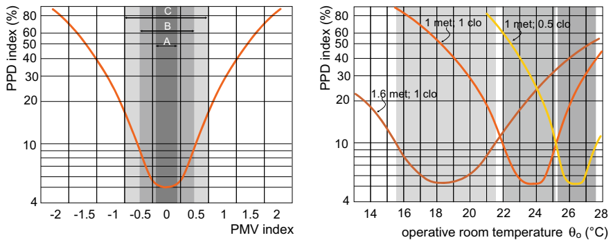
Fig. 1.112 PPD index vs. PMV index as determined by Prof. Fanger in the 1980s (left). It is assumed that even in a thermally neutral environment ( PMV\ 0 ), 5% of people will be dissatisfied with their indoor thermal comfort. The curve in the figure on the left is given for a seated person (1.2 met) wearing light clothes (1.0 clo). The range of the operative temperature \theta_o at which the PPD index will be lower than 10% at different activity met and clothing clo of the person in the room (right). The PPD is determined for v\ 0.15\ \text{m/s} and a relative air humidity \varphi_i\ 50\% [33]
