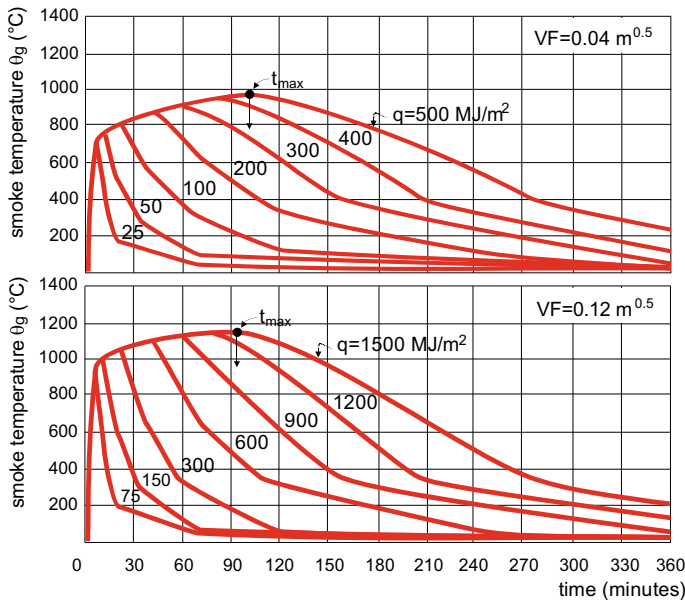
Fig. 6.22 Fire-compartment EUROCODE temperature \theta_g -time curves for different specific heat releases q ( \text{MJ/m}^2 ), above for ventilation factor VF = 0.04 \text{ m}^{1/2} , below for ventilation factor VF = 0.12 \text{ m}^{1/2} . In both cases it was assumed that the thermal effusivity of the building structures is 1160 \text{ J/m}^2\text{Ks}^{1/2}
