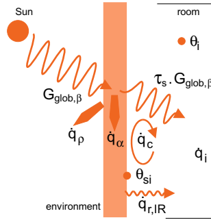
Fig. 1.56 Total heat flux q_i entering the room due to the insolation of the window equals the sum of the transmitted solar radiation \tau_s \cdot G_{glob,\beta} , the convective heat flux \dot{q}_c and the long-wave heat flux \dot{q}_{r,IR} transferred into the room from the internal surface of the glazing. The ratio of these heat fluxes determines the total solar energy transmittance of the glazing g
