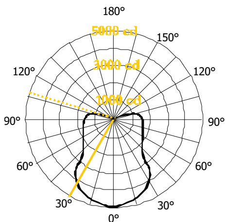
Fig. 4.11 The candela diagram for the point-type luminaire. The luminous intensity of the luminaire in the direction towards down (angle 0^\circ ) is 5000 cd, while in the direction 30^\circ from the vertical it is 4000 cd. If there will be no reflection of the light on the surfaces in the room, the ceiling of the room will be unlighted because the luminaire does not emit light in the space at an angle greater than 107^\circ from the vertical direction
