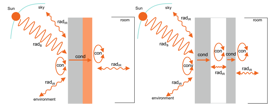
Fig. 1.30 Heat fluxes in opaque building structures (left); heat fluxes in opaque building structure with close cavity (right); cond—conduction, con—convection, rad_s —short wavelength solar radiation, rad_{IR} —long wavelength (IR) radiation
