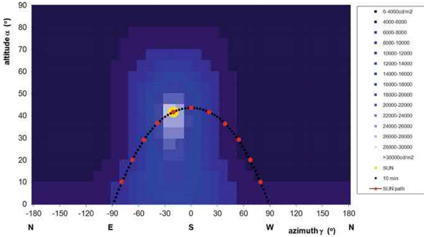
Fig. 4.31 Luminance of patches in the sky determined for clear sky conditions. The sun path is shown for the 21st of March for a location with the geographical latitude L 46^\circ and the illuminance of the sky is shown for 11 o'clock on the same day [14]
