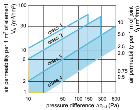
Fig. 2.17 Amount of air passing through the joints of the door or window at pressure differences \Delta p_{e-i} expressed per 1 m 2 of element area or per 1 m of joint between the frame and sash length in one hour. Values define the airtightness class of the window or door at a pre-defined pressure difference (100 Pa) [13]
