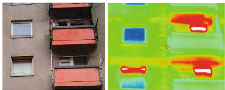
Fig. 2.18 Thermal image of the building confirms the findings from the case study. After the replacement of the windows, the tenants are very often leaving windows open in bathrooms over the night. IR image confirms high heat losses due ventilation in such case [14]
