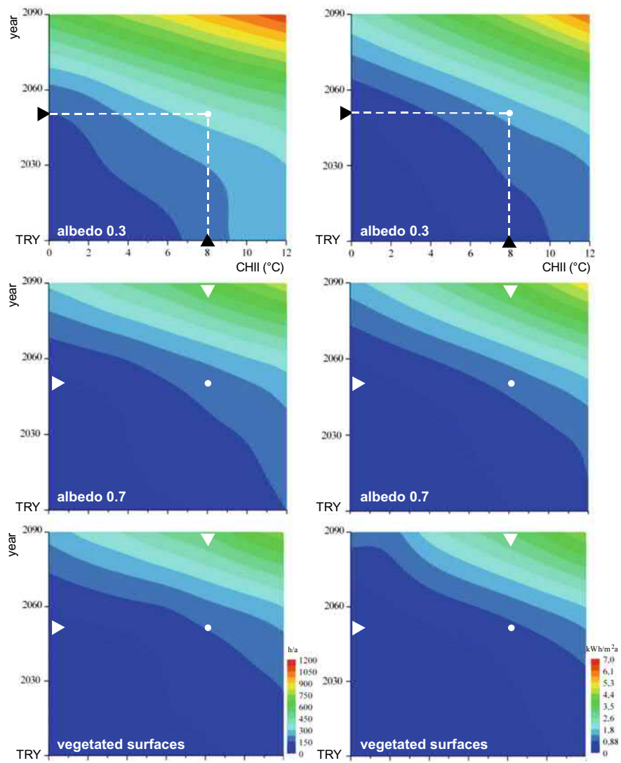
Fig. 7.17 Number of overheating hours OHH (h/year) when indoor-air temperature exceeds the thermal comfort limit ( \theta_i = > 26\text{ }^{\circ}\text{C} ) (left) and predicted increase in specific energy needs for cooling ( \Delta Q_{C,nd} in \text{kWh/m}^2\text{a} ) (right) versus street-canyon heat-island intensity CHII from present to 2090; values are shown for the dark building blocks (albedo 0.3), light coloured building blocks (albedo 0.7) and street canyon with vegetated surfaces; mid-severe global climate change scenario (+ 4.5 K) was taking into account; drawn point shown predicted OHH and \Delta Q_{C,nd} in 2050 and CHII 8 K [26].
