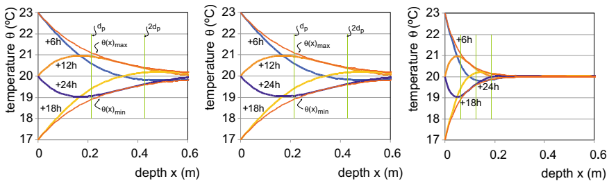
Fig. 1.98 Thermal response of a thermal insulation layer (thermal diffusivity a = 167.10^{-8} \text{ m}^2/\text{s} , left), a concrete ( a = 68.10^{-8} \text{ m}^2/\text{s} , middle) and a wooden ( a = 14.10^{-8} \text{ m}^2/\text{s} , right) building structure of infinite thickness to a periodic change in the surface temperature; \theta_{se} = 20^\circ \text{C} , \theta_a = 3 \text{ K} , t_0 = 0 \text{ h} , t_0 = 24 \text{ h}
