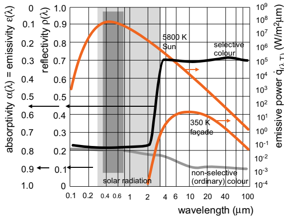
Fig. 1.22 Radiative properties of the surface of the façade painted with a non-selective and a selective paint. Because the reflectivity of the light is the same for both surfaces, the shade of the surface colour will be the same, while the heat flux emitted by the selective surface will be significantly lower due to the lower emissivity of the long-wavelength thermal radiation
