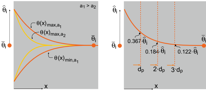
Fig. 1.97 Thermal response zone of a building structure with infinite thickness to a periodic change of the surface temperature depends on the thermal diffusivity of matter a . The envelope curves \theta(x)_{\max,a} and \theta(x)_{\min,a} —showing the cases where a_1 is greater than a_2 —determine the volume of the building structure inside which the temperature over the period t_p periodically changes (left). The periodic heat-penetration depth d_p (m) is the depth of the structure at which the amplitude of the temperature decreases by a factor 1/e of the amplitude of the indoor-air temperature \hat{\theta}_{i,(x=0)} , while at a double periodic heat-penetration depth the amplitude of the temperature decreases by a factor 1/(2 \cdot e) and at a triple heat-periodic penetration depth by the factor 1/(3 \cdot e) of the amplitude of the indoor-air temperature \hat{\theta}_{i,(x=0)} ; (right)
