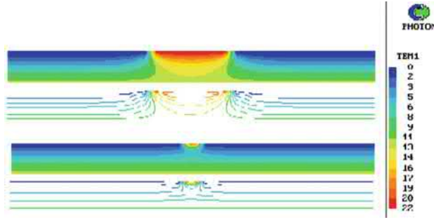
Fig. 1.65 Temperature distribution in the ground under a 50 \times 50 \text{ m}^2 and a 10 \times 10 \text{ m}^2 building, down to a depth of 50 m. The thermal losses through the building structures in contact with the ground are considerably smaller than the losses into the air through building structures at the building envelope. Due to a large affected zone, the numerical simulation of heat transfer through the structures in contact with the ground must consider the ground volume, a multiple of the building volume
