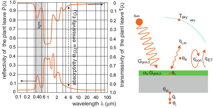
Fig. 1.60 Radiative properties of plant leaves are adapted to the absorption of wavelengths involved in photosynthesis ( \sim 0.43 and \sim 0.66 \mu\text{m} ), while the leaves have a high reflectivity with respect to the thermal part of the solar radiation ( 0.78 < \lambda < 3 \mu\text{m} ) and a high emissivity of thermal radiation ( \lambda > 3 \mu\text{m} ), which reduces the overheating of the leaves (left). The vegetation blanket temperature \theta_v is determined by the energy balance of the heat fluxes. The greened structures differ with respect to the others by the evapo-transpiration heat flux \dot{q}_{ET} , with which a major part of the absorber solar irradiation by the leaves ( \alpha_s \times G_{\text{glob},\beta} ) is transferred from the plant to the surroundings. Because of this, the temperature of the vegetation blanket is very close to the temperature of the outdoor air \theta_e even in case of high solar irradiation (right)
