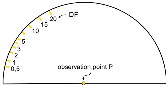
Fig. 4.55 The protractor method is based on a graphical tool on which the sky component DF can be read for any selected point in the room; the standard CIE overcast sky model is used [16]
