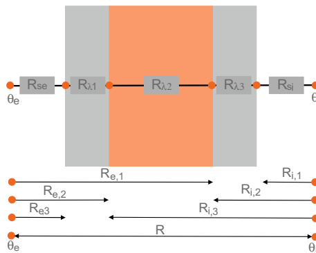
Fig. 1.83 The principle for the determination of the resistance to the heat transfer R_{i,c} on the inner part and R_{e,c} on the external part of the building structure in the case of building structure with 3 layers
