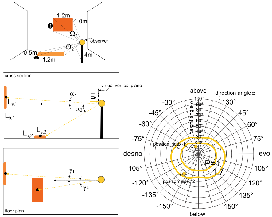
Fig. 4.70 Height angles and direction angles from the case study (left); position index of the observer P towards the window and the sunlit floor (right)
