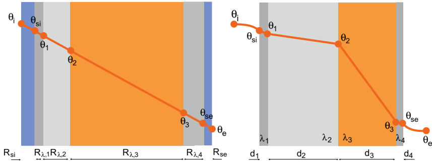
Fig. 1.38 Temperature distribution in a homogeneous building structure when the thicknesses of the layers are replaced by their resistances to heat transfer (left). The actual temperature distribution in the same building structures (right)
