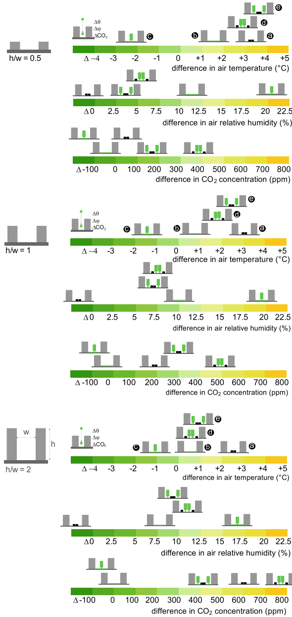
Fig. 7.16 Difference between the street canyon's and rural surrounding's air temperature ( \Delta\theta_e ), relative air humidity ( \Delta\phi_e ) and concentration of CO 2 ( \Delta CO_2 ) at the level of pedestrian. Cases are shown for: a the street canyon with road, b the street canyon with grassy ground, c street canyon with a tree-lined avenue, d street canyon with two-way traffic and tree-lined avenue along the sides of the street and e the street canyon with two-way traffic and tree-lined avenue in the middle of the canyon. Three examples are presented according to the street canyon height-to-width ( h/w ) ratio [25]
