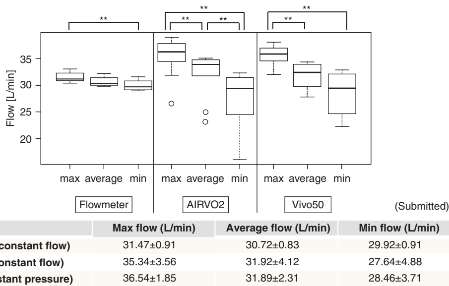
Fig. 10.1 Comparison of the flow rate between constant flow and constant pressure
