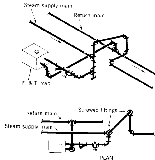
Fig 15-32. Swing type expansion loop combined with main rise and drip
