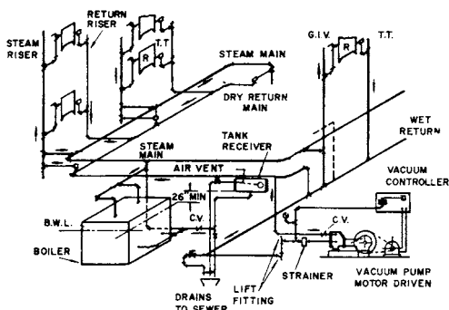
Fig 15-66. Mechanical vacuum system
