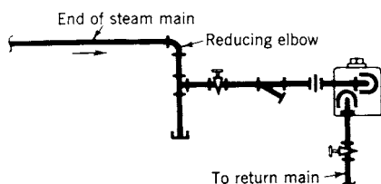
Fig 15-19. Details of end of main drip
