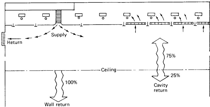
Fig 13-53. Proportionate heat distribution through luminous or louvered ceiling
