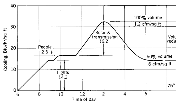
Fig 13-43. Load profile
