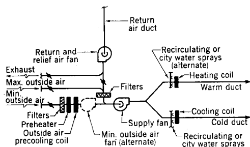
Fig 13-90. Single fan dual duct cycle with additional minimum outside air dehumidifier
