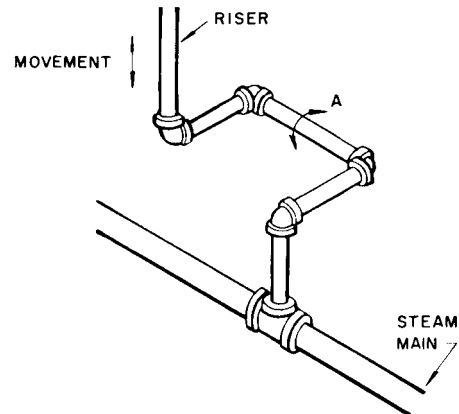
Fig 15-40. Riser connected to allow for expansion
