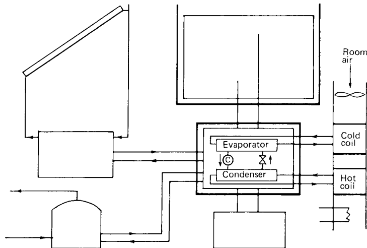
Fig 13-87. Dehumidification
