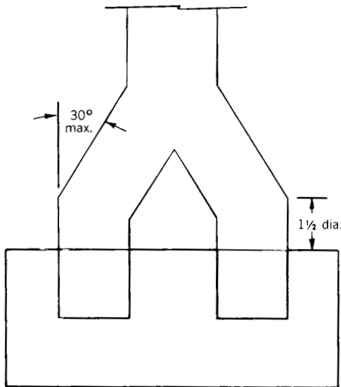
Fig 14-52. Proper construction of a pants connection on a two-fan unit
