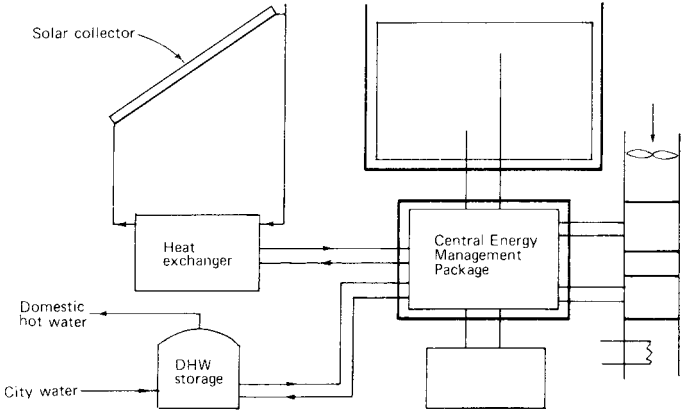
Fig 13-79. Solar heating of domestic hot water
