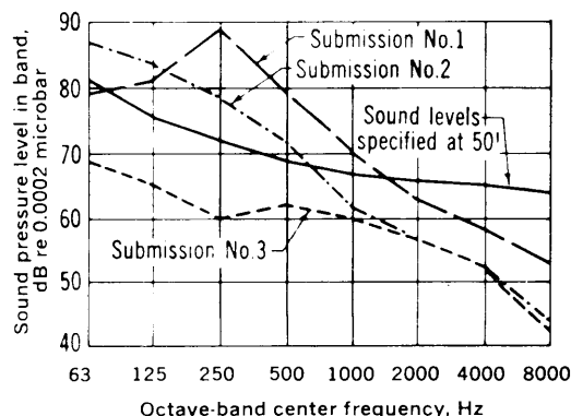
Fig 16-30. Manufacturers cooling tower submissions to meet sound level specifications
