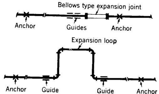
Fig 15-31. Expansion joint detail
