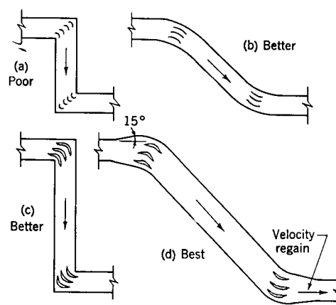
Fig 14-71. Air stream turns between successive fittings
