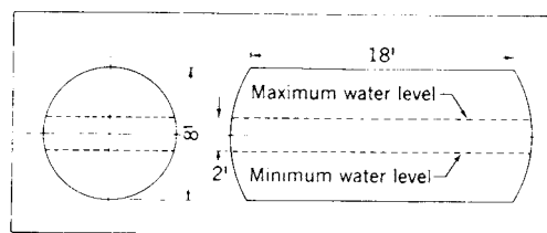
Fig 15-113. Horizontal steam pressurizing tank
