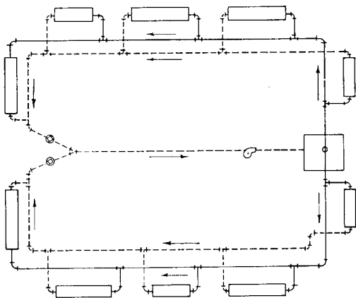
Fig 15-96. Two pipe reversed return system
