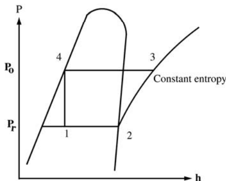
Fig 1-5b. Practical refrigeration cycle in P-h coordinates
