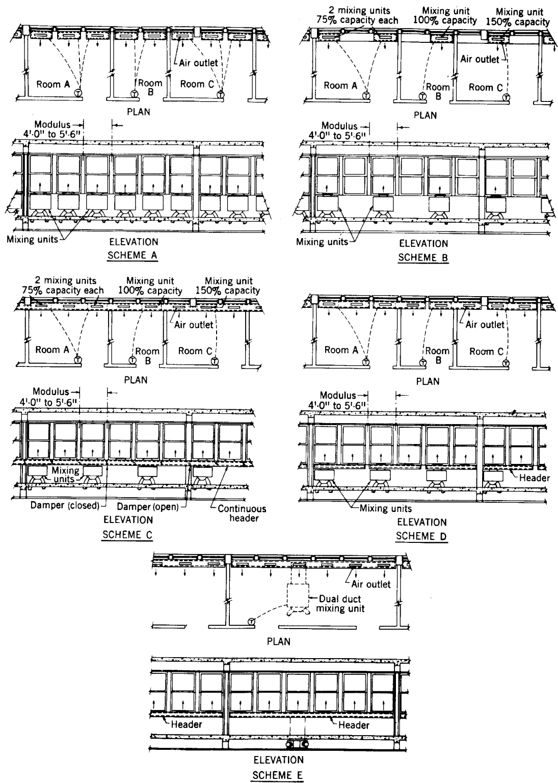
Fig 13-108. Modular arrangement of dual duct mixing units
