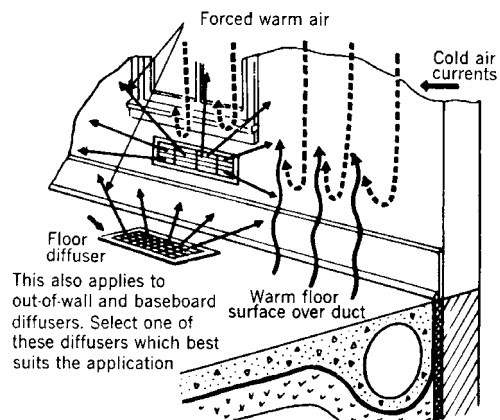
Fig 15-135b. Details of perimeter loop system with floor or baseboard diffuser below window
