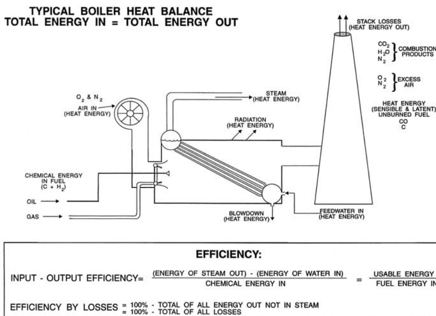
Fig 12-4. Typical boiler heat balance
