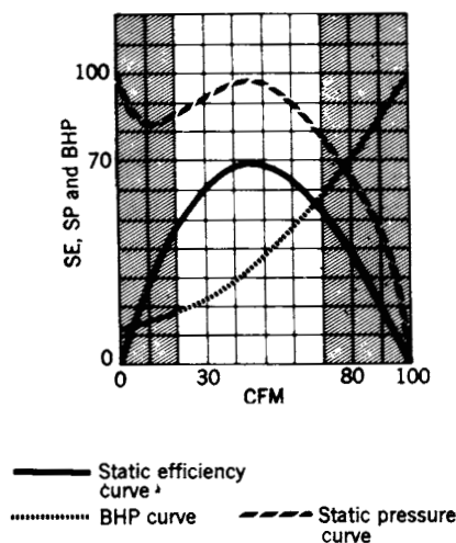
Fig 14-33. Characteristic curve for FC fans
