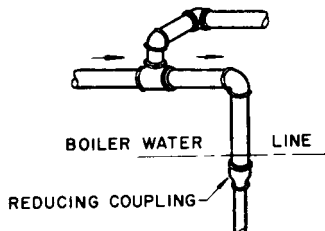
Fig 15-44. Dripping steam main
