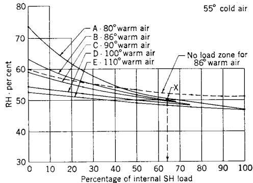
Fig 13-96. Performance over rate of internal sensible heat load; system of Figs. 13-88 and 13-89 for 55°F cold air
