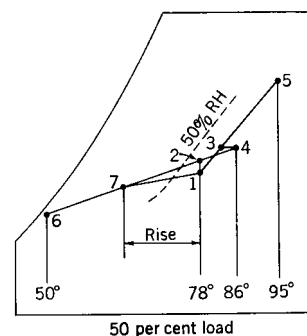
Fig 13-94. Psychrometric chart for dual duct system for Fig. 13-88 50% load
