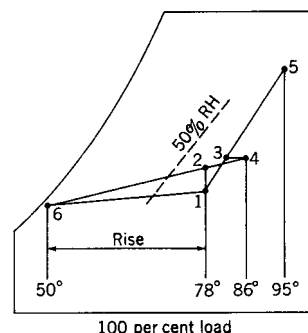
Fig 13-93. Psychrometric chart for dual duct system for Fig. 13-88 full load
