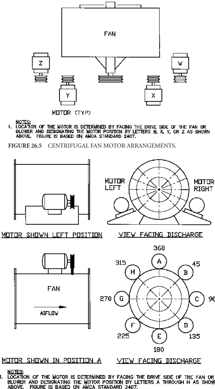
FIGURE 26.6 INLINE FAN MOTOR ARRANGEMENTS.
