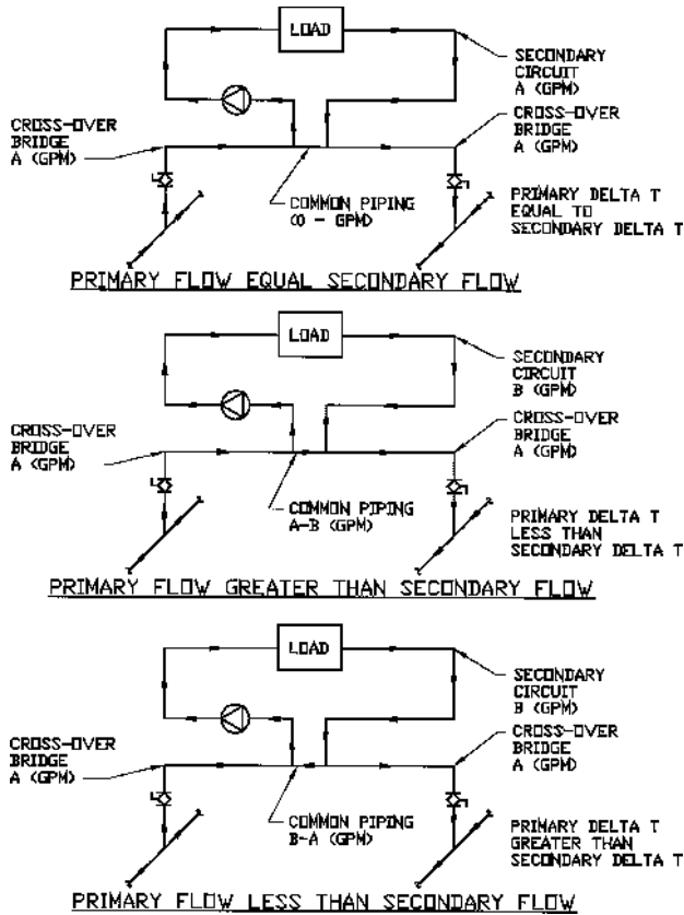
FIGURE 19.13 PRIMARY-SECONDARY FLOW ANALYSIS.
