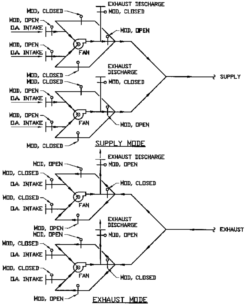
FIGURE 26.16 DWDI CENTRIFUGAL FANS (REVERSIBLE FLOW).
