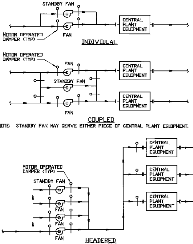
FIGURE 26.3 STANDBY FANS.
