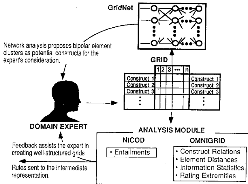
FIGURE 7. The repertory grid components of ICONKAT.
